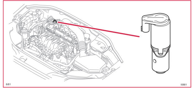
8/81 Reset valve, camshaft exhaust, 4-Cyl.
