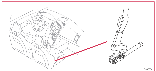
8/93 Lap belt tensioner, passenger
