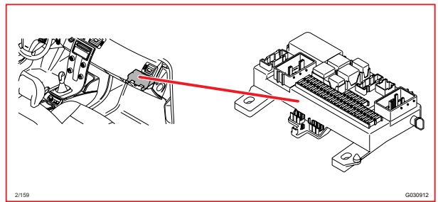
2/159 Relais Infotainment
